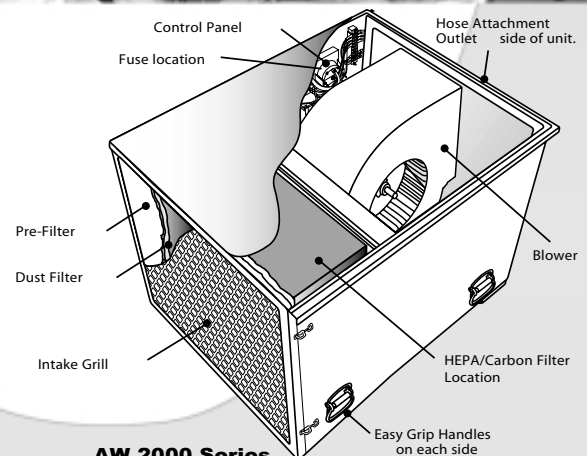
AW 2000 Series Detailed schematic.
